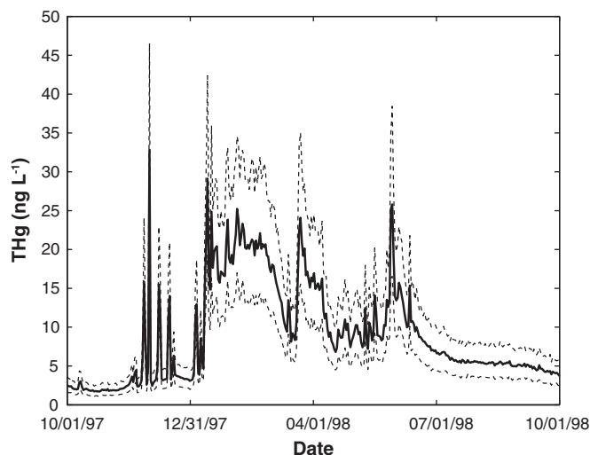
Fig. 6. Example of the second stage prediction of daily mercury concentration (bold line) and 90% confidence interval, Sacramento River at Colusa, water year 1998.
