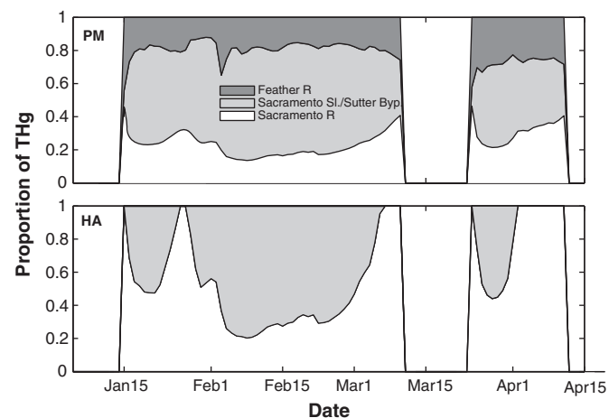
Fig. 4. Relative contributions of THg in flow from three sources over Fremont Weir under PM (top) and HA (bottom) for a flooding period in 1998.
